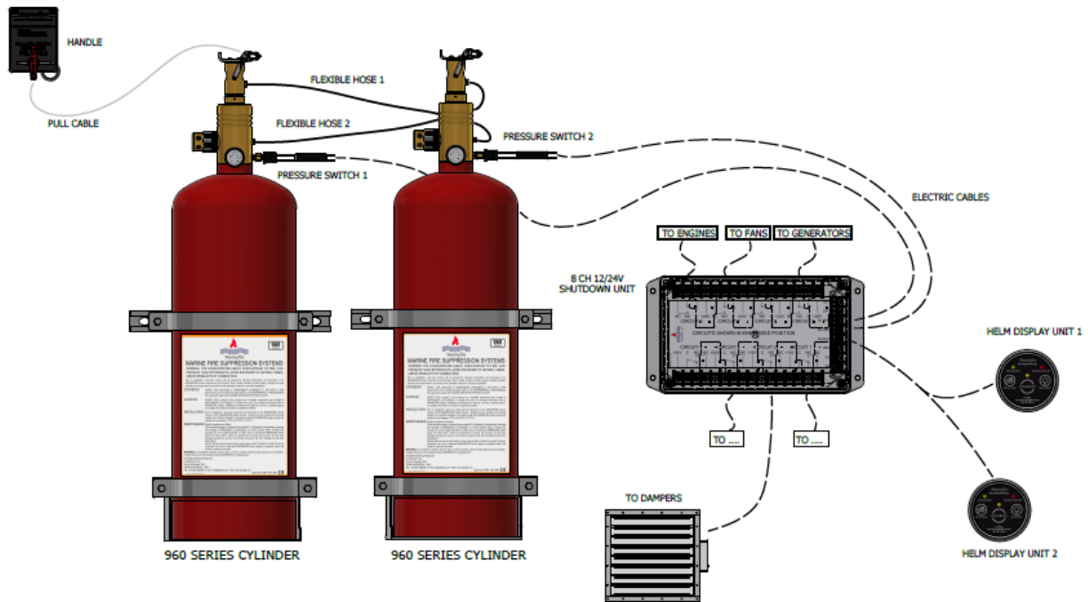
Two cylinders configuration
