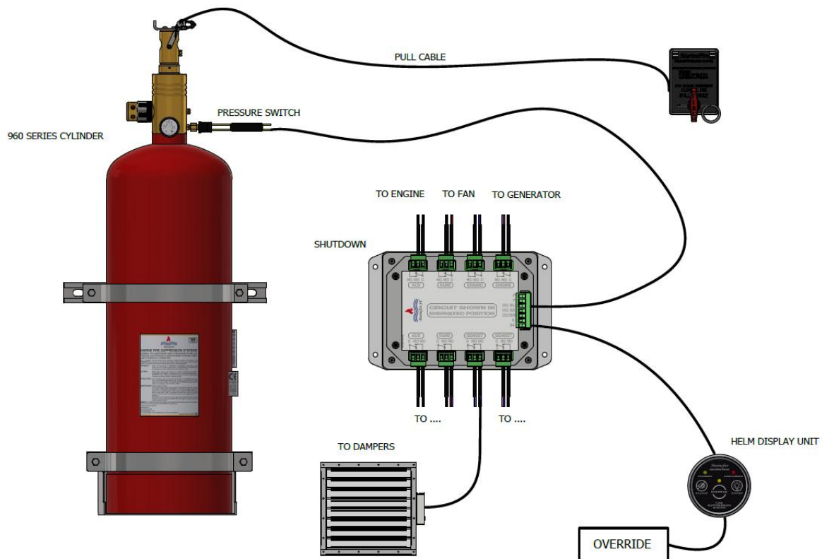
Single cylinder configuration
