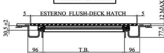
PLEXIGLASS PIANO
