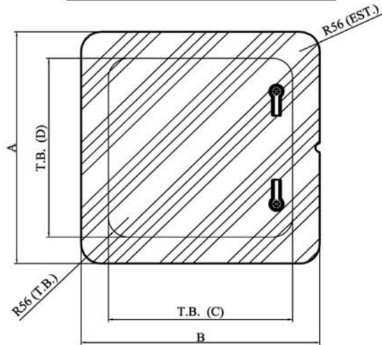
PLEXIGLASS CURVO
