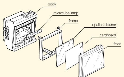
Microtube lamp and customized cardboard assembly
