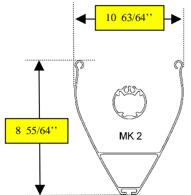
Mk2 boom section
