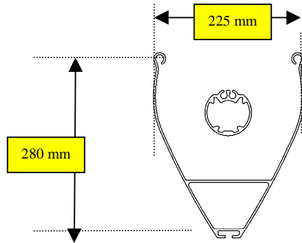
Section de bôme MK 2R
